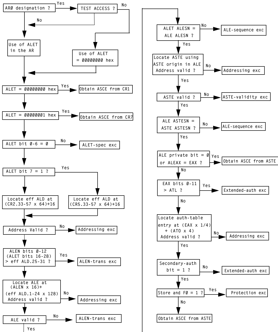
Figure 5-14. Access-Register-Translation Steps and Exceptions
