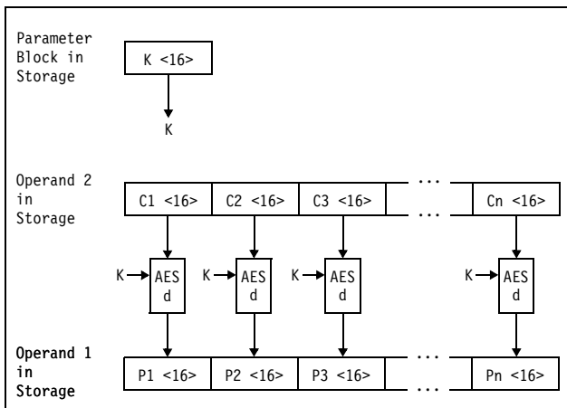
Figure 7-21. KM-AES-128 Decipher Operation
