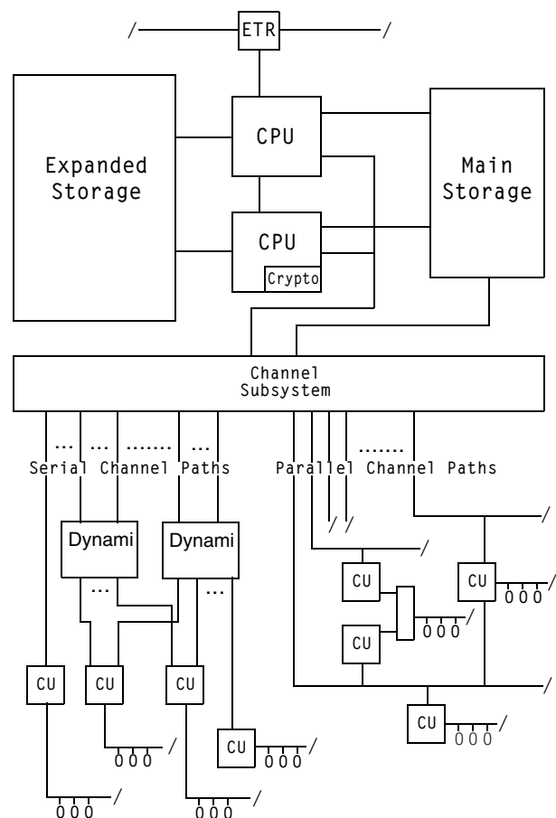
Figure 2-1. Logical Structure of a z/Architecture System with Two CPUs
