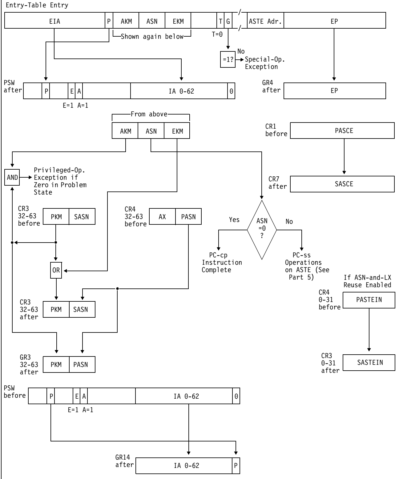
Figure 10-37. Execution of PROGRAM CALL (Part 2 of 5).
