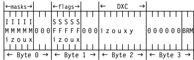
Figure 19-1. FPC Register Overview
