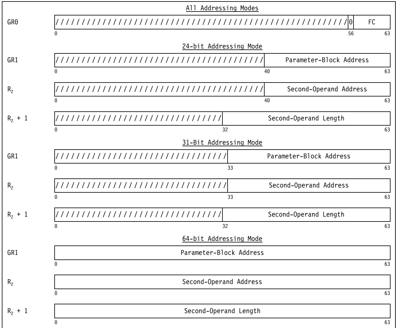
Figure 7-72. General Register Assignment for KMAC
