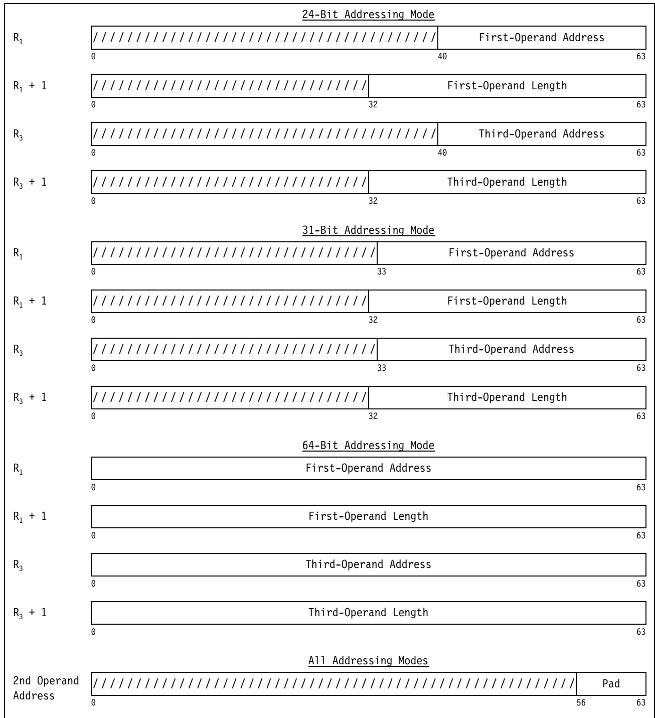
Figure 7-90. Register Contents and Second-Operand Address for MOVE LONG EXTENDED
