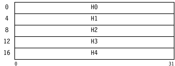
Figure 7-55. Parameter Block for KIMD-SHA-1
