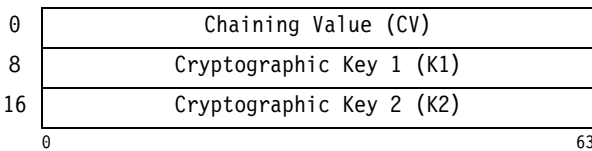
Figure 7-78. Parameter Block for KMAC-TDEA-128
