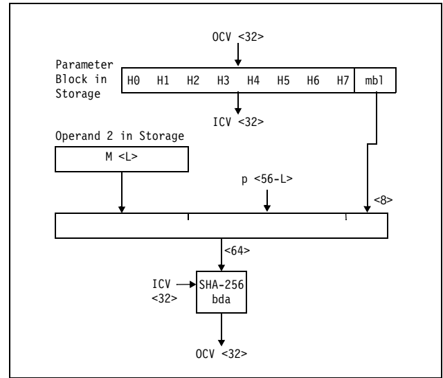
Figure 7-68. KLMD-SHA-256 Partial-Block Case 1 ( 1 \leq L \leq 55 )
