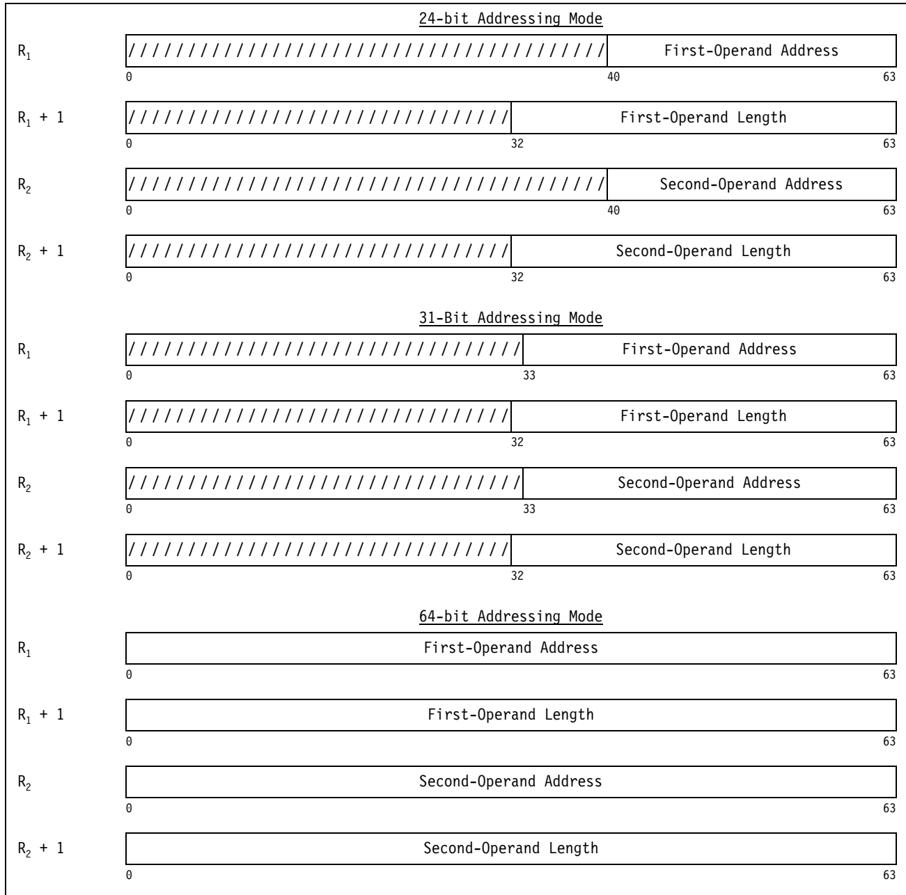
Figure 7-86. Register Contents for CONVERT UTF-32 TO UTF-8
