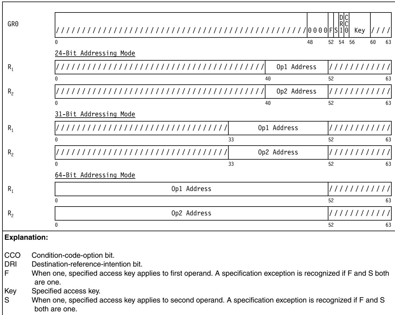
Figure 10-20. Register Contents for MOVE PAGE
