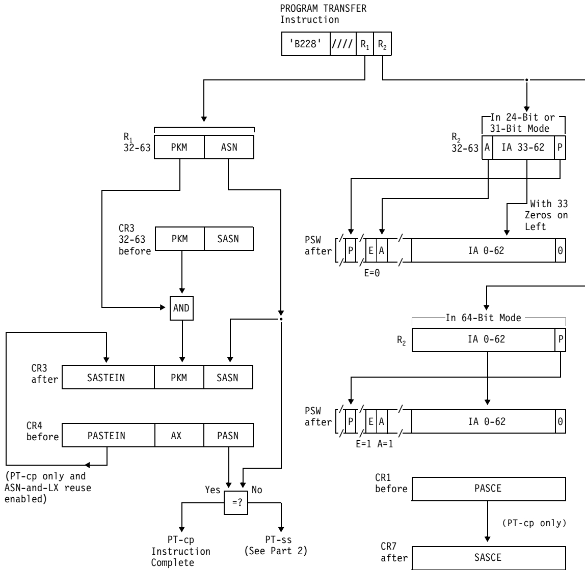
Figure 10-40. Execution of PROGRAM TRANSFER (Part 1 of 2).
