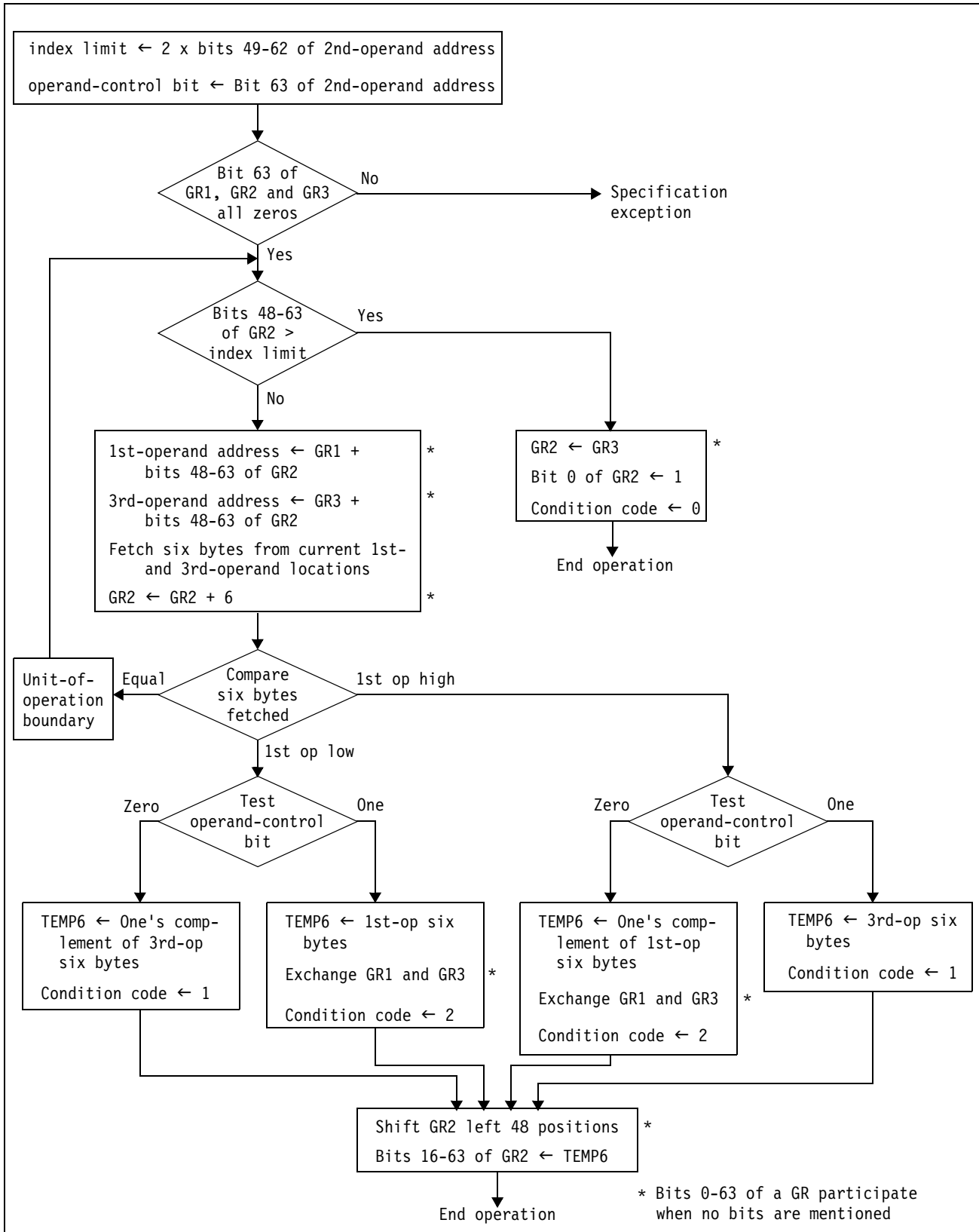
Figure 7-41. Execution of COMPARE AND FORM CODEWORD in the 64-bit Addressing Mode
