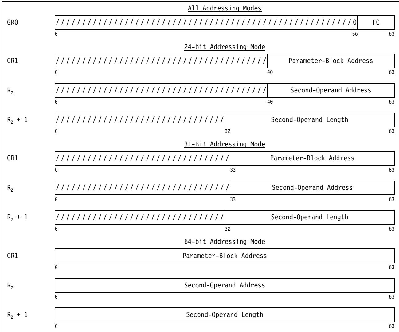
Figure 7-51. General Register Assignment for KIMD and KLMD
