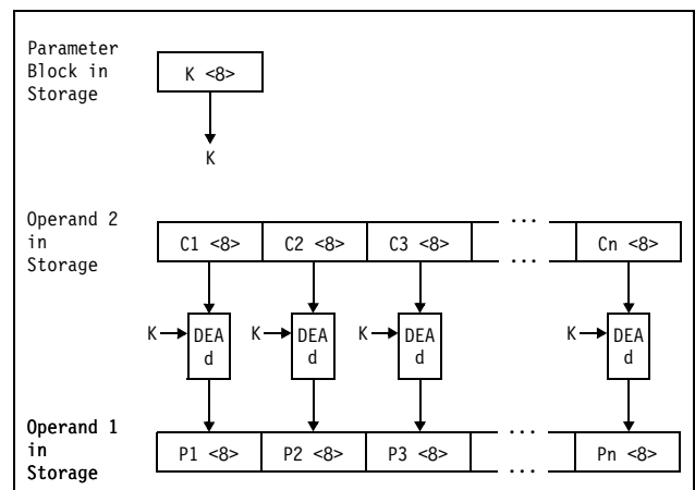
Figure 7-12. KM-DEA Decipher Operation
