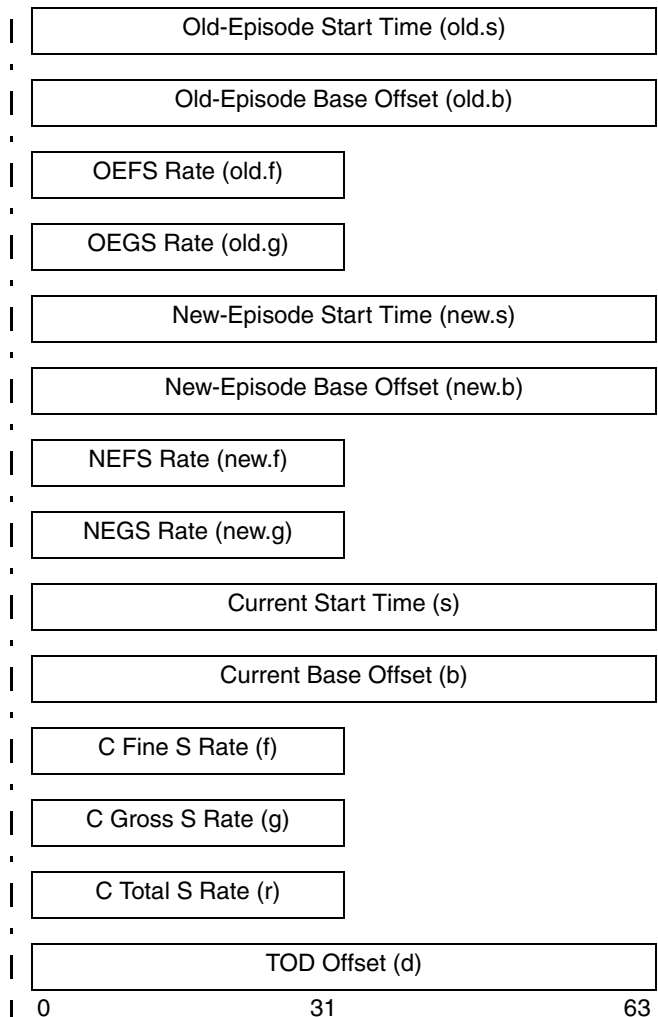
Figure 4-11. TOD-Clock-Steering Registers
