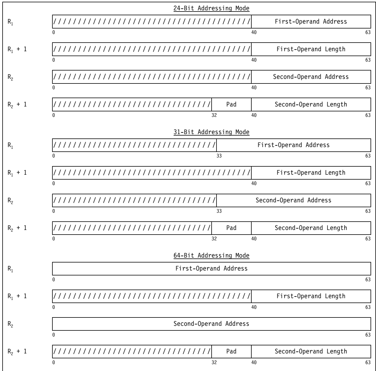
Figure 7-89. Register Contents for MOVE LONG
