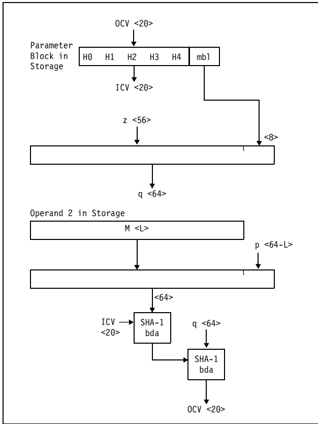
Figure 7-64. KLMD-SHA-1 Partial-Block Case 2 ( 56 \leq L \leq 63 )
