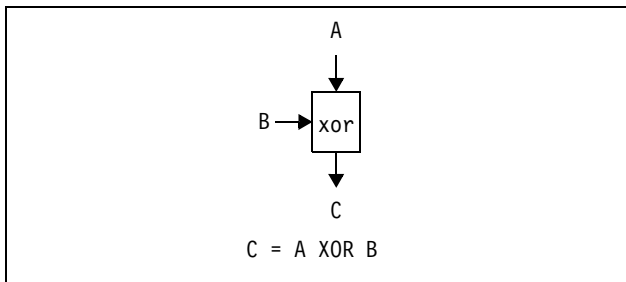
Figure 7-73. Symbol For Bit-Wise Exclusive OR
