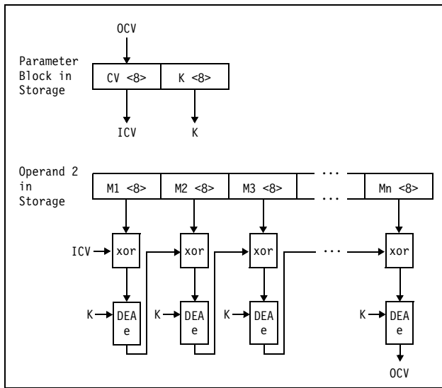
Figure 7-77. KMAC-DEA
