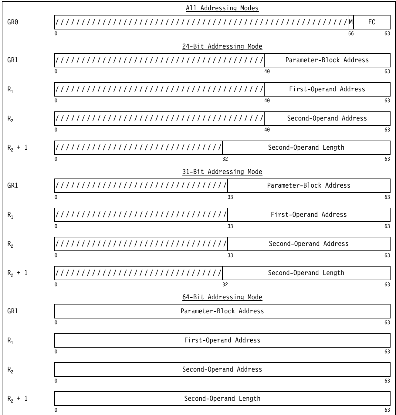
Figure 7-5. General Register Assignment for KM and KMC
