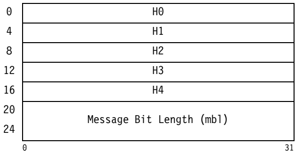
Figure 7-60. Parameter Block for KLMD-SHA-1
