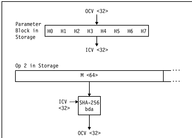
Figure 7-66. KLMD-SHA-256 Full Block ( L \geq 64 )
