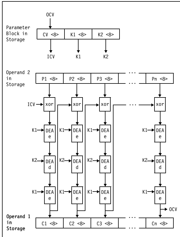
Figure 7-27. KMC-TDEA-128 Encipher Operation
