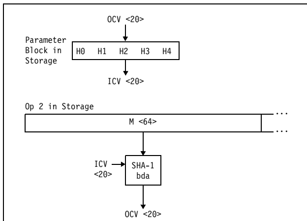
Figure 7-61. KLMD-SHA-1 Full Block ( L \geq 64 )
