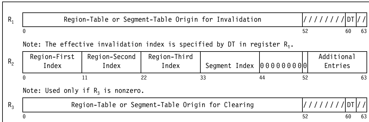
Figure 10-12. Register Contents for INVALIDATE DAT TABLE ENTRY Invalidation-and-Clearing Operation (Bit 52 of GR R_2 Is Zero)
