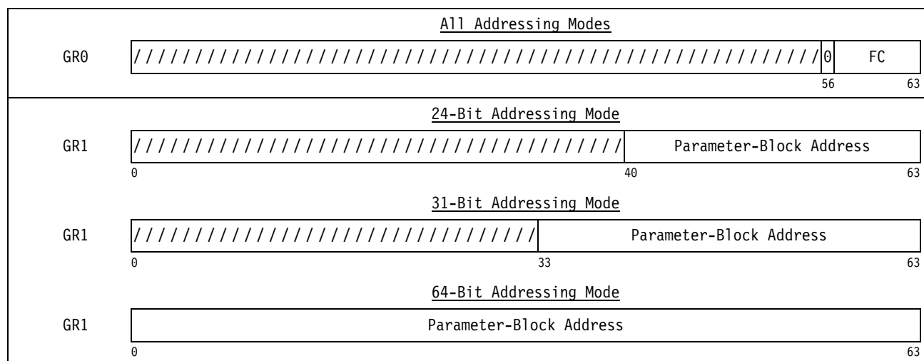
Figure 10-23. General Register Assignment for PERFORM TIMING FACILITY FUNCTION
