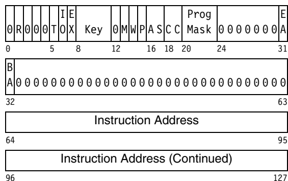
Figure 4-2. PSW Format
