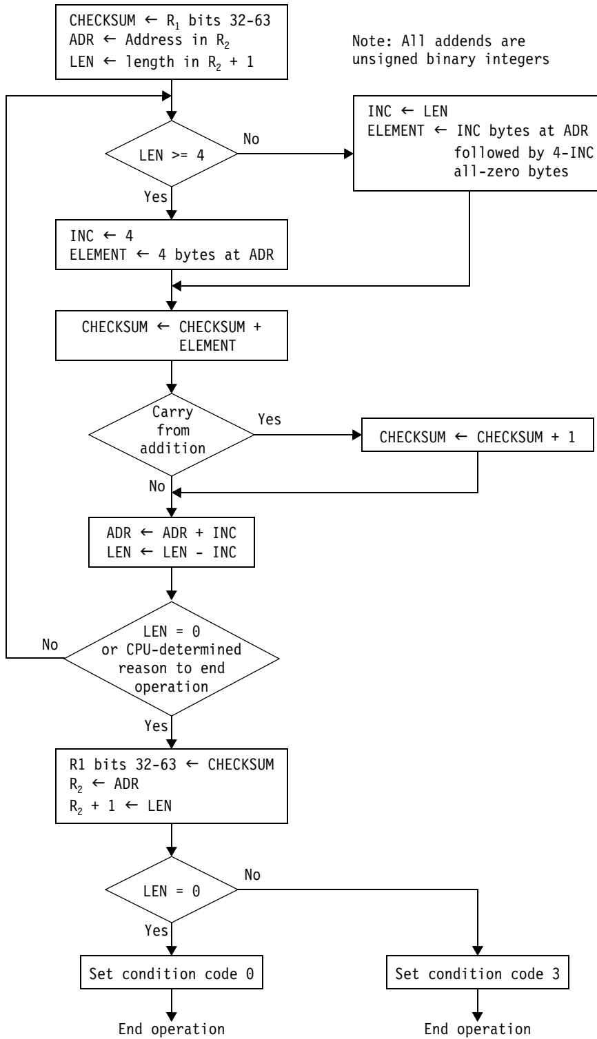
Figure 7-2. Execution of CHECKSUM
