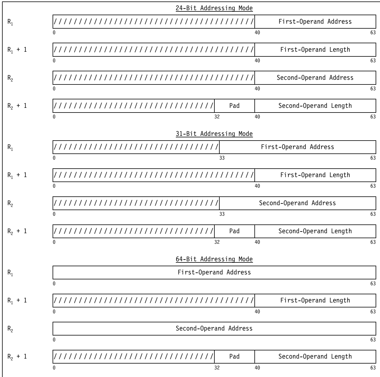
Figure 7-42. Register Contents for COMPARE LOGICAL LONG
