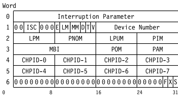
Figure 15-1. PMCW Format
