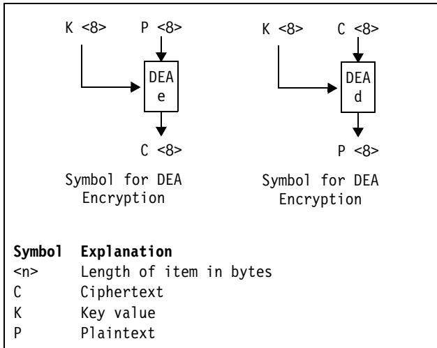
Figure 7-74. Symbols for DEA Encryption and Decryption
