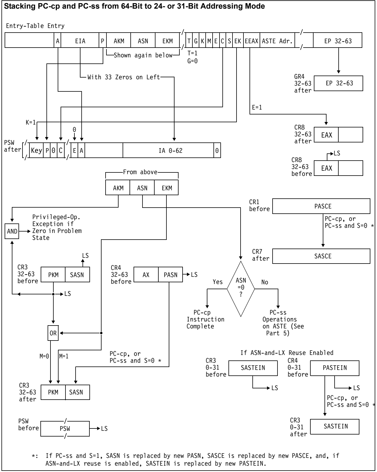
Figure 10-37. Execution of PROGRAM CALL (Part 4 of 5).
