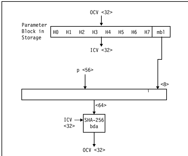
Figure 7-67. KLMD-SHA-256 Empty Block ( L = 0 )
