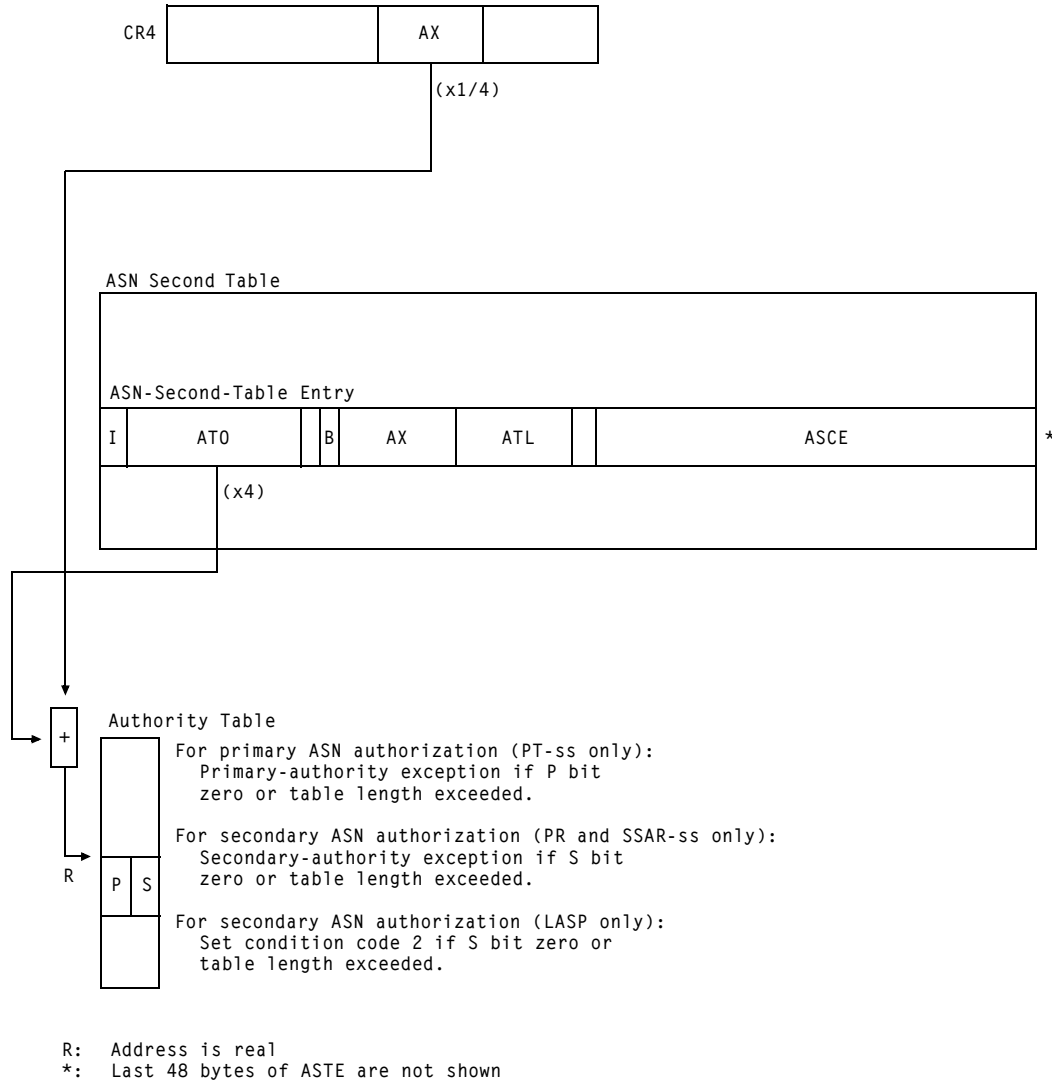
Figure 3-8. ASN Authorization
