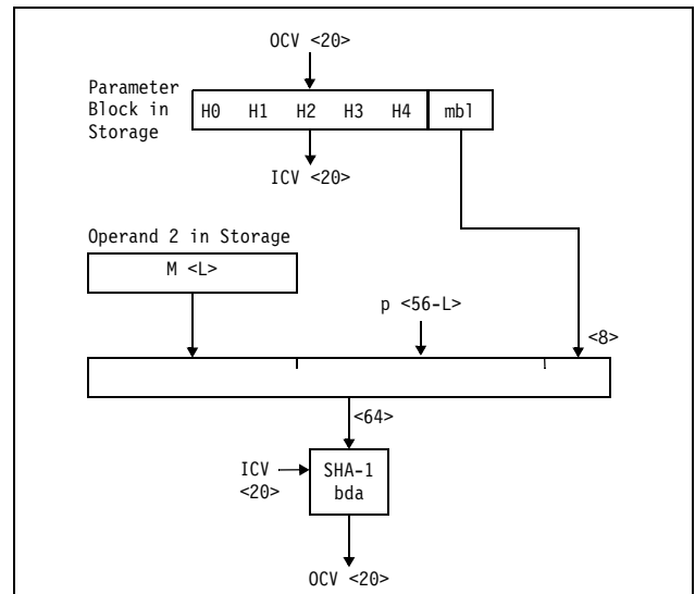
Figure 7-63. KLMD-SHA-1 Partial-Block Case 1 ( 1 \leq L \leq 55 )
