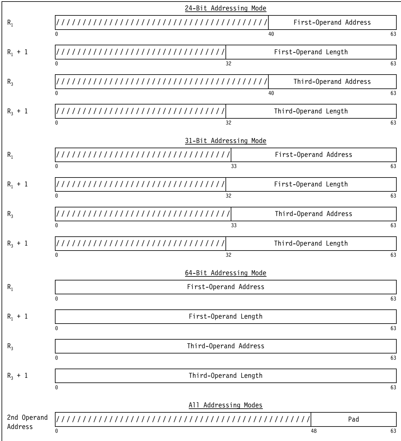
Figure 7-44. Register Contents and Second-Operand Address for COMPARE LOGICAL LONG UNICODE
