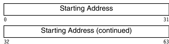
Control Register 10
