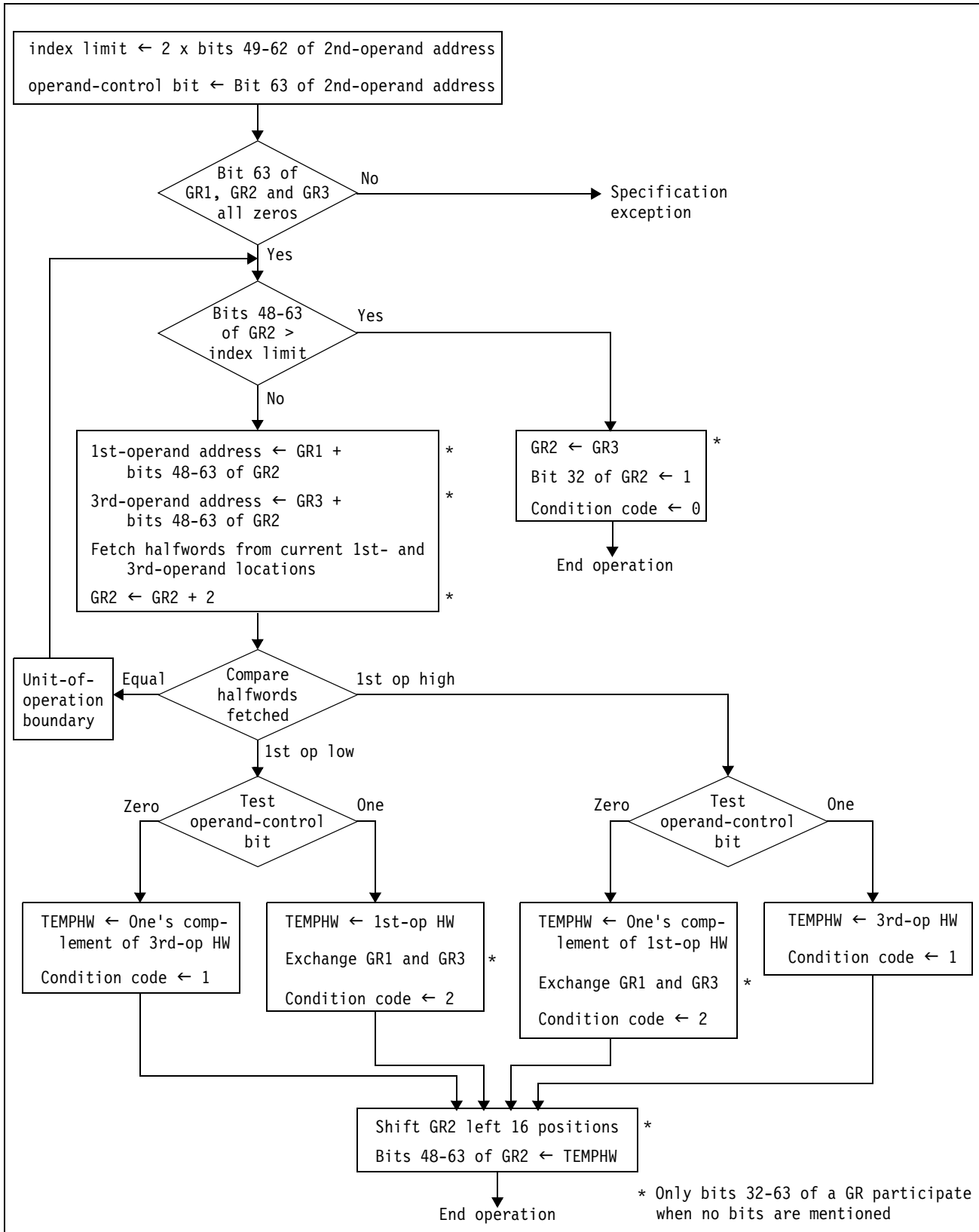
Figure 7-39. Execution of COMPARE AND FORM CODEWORD in the 24-Bit or 31-bit Addressing Mode
