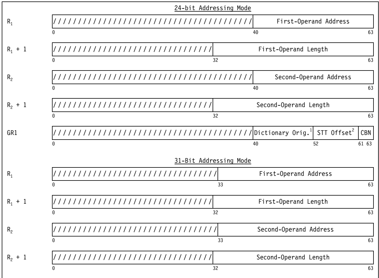
Figure 7-46. Register Contents for COMPRESSION CALL (Part 1 of 2)
