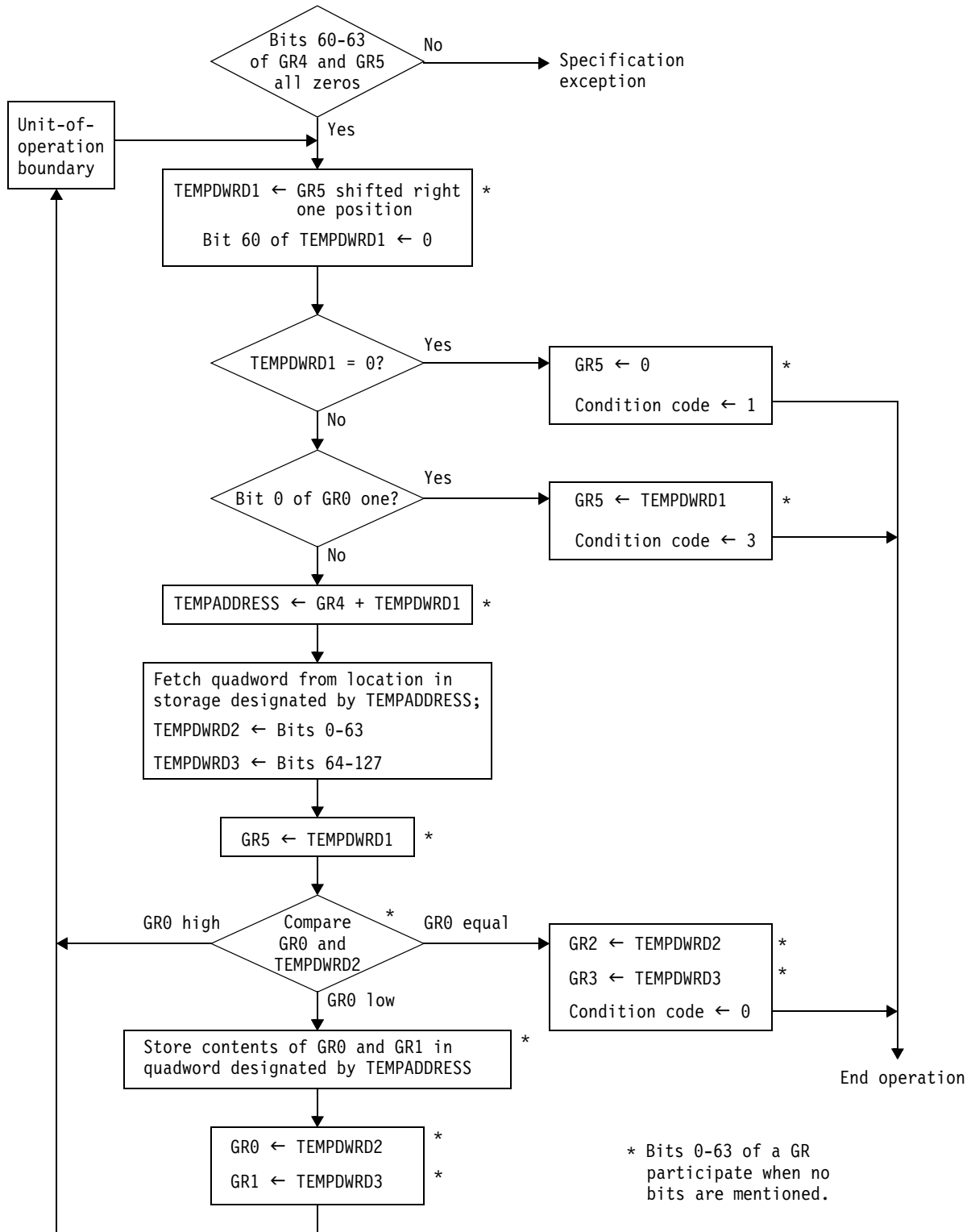
Figure 7-99. Execution of UPDATE TREE in the 64-Bit Addressing Mode
