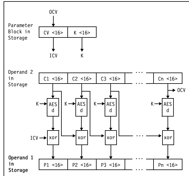
Figure 7-34. KMC-AES-128 Decipher Operation
