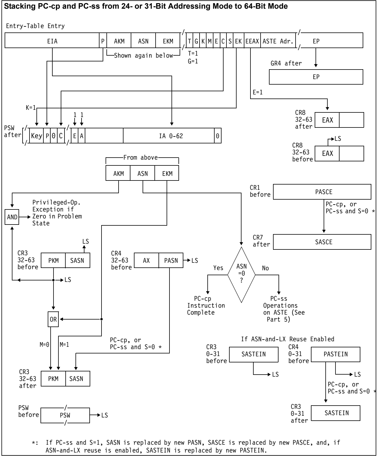
Figure 10-37. Execution of PROGRAM CALL (Part 3 of 5).
