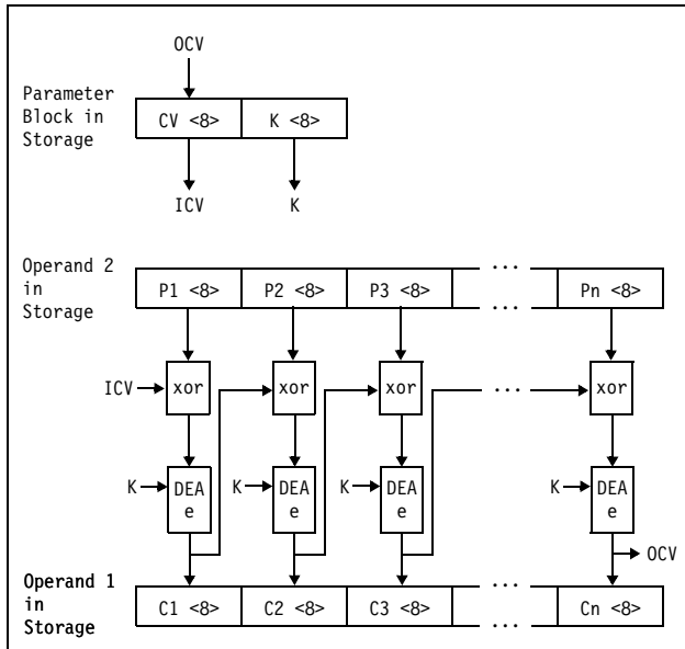
Figure 7-24. KMC-DEA Encipher Operation
