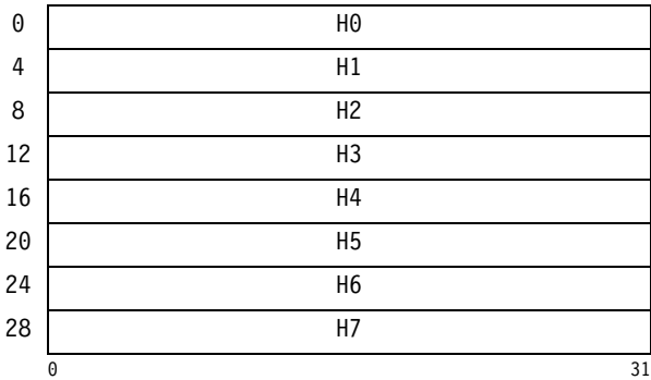
Figure 7-57. Parameter Block for KIMD-SHA-256
