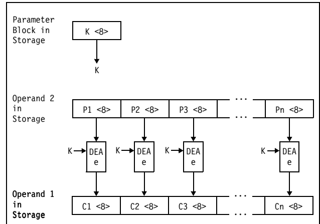
Figure 7-11. KM-DEA Encipher Operation
