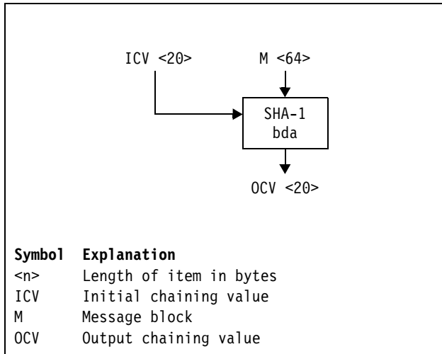
Figure 7-52. Symbol for SHA-1 Block Digest Algorithm
