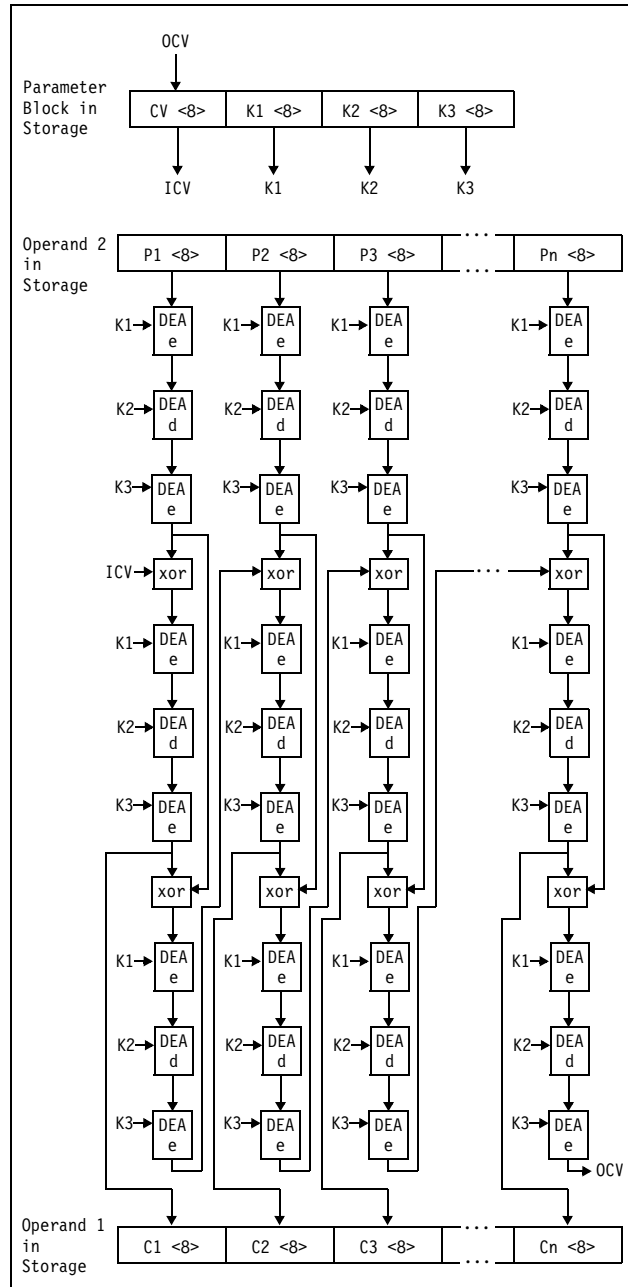
Figure 7-36. KMC-PRNG
