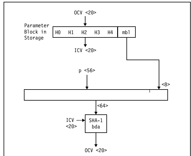
Figure 7-62. KLMD-SHA-1 Empty Block ( L = 0 )
