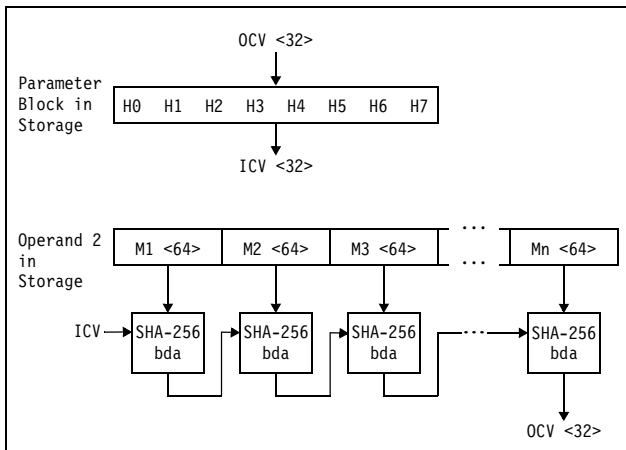
Figure 7-58. KIMD-SHA-256
