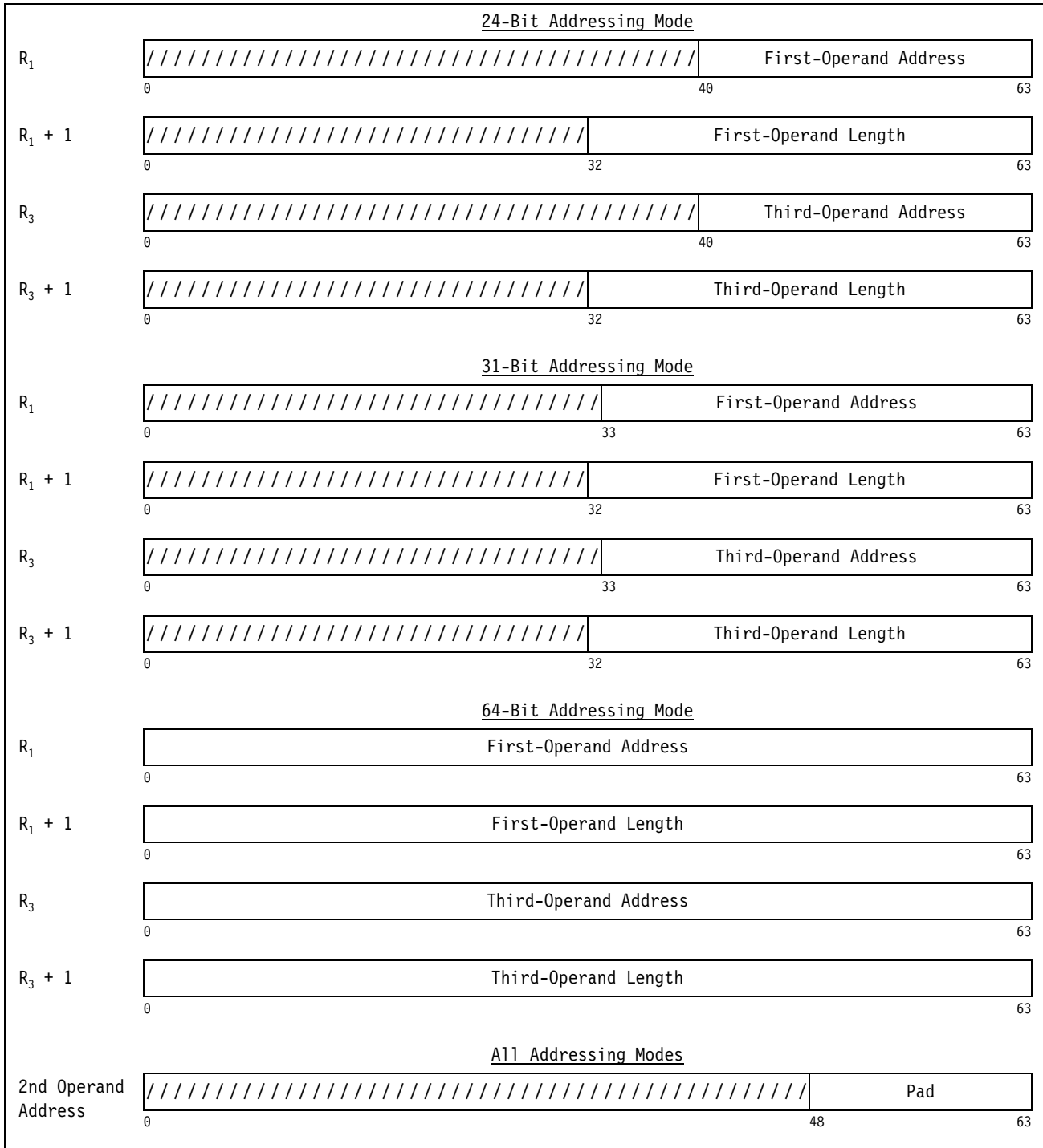
Figure 7-91. Register Contents and Second-Operand Address for MOVE LONG UNICODE
