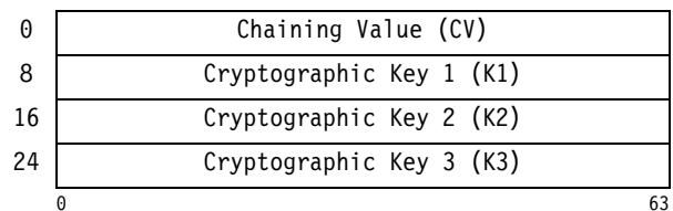
Figure 7-80. Parameter Block for KMAC-TDEA-192
