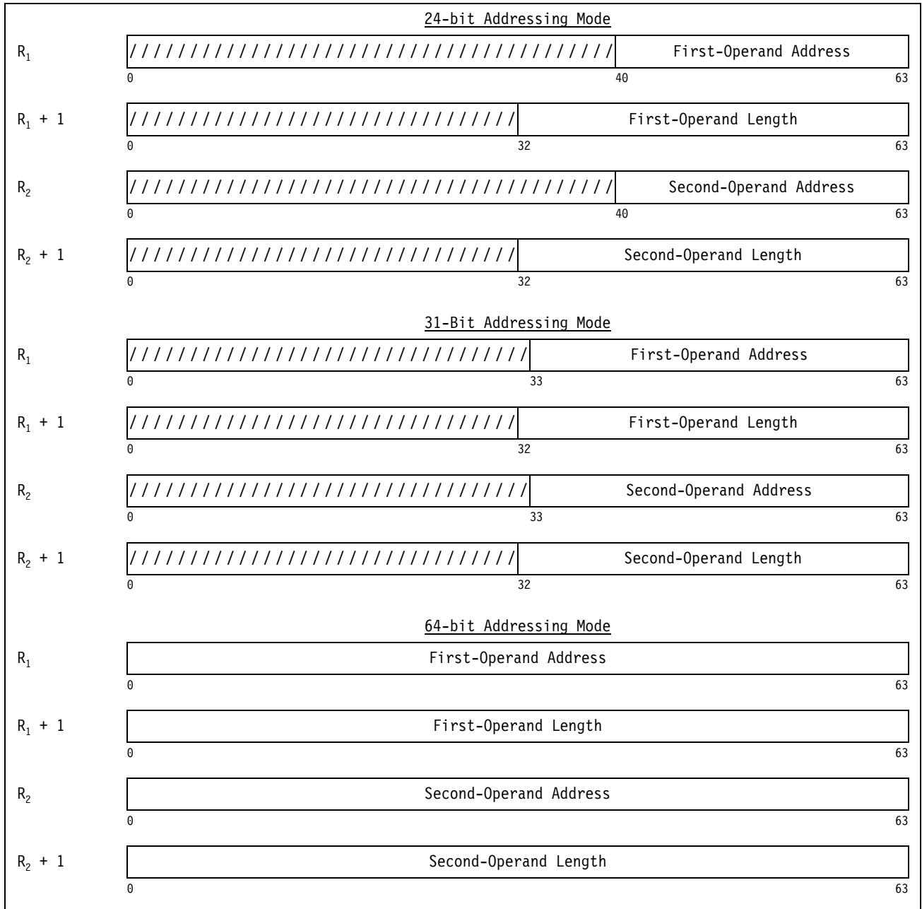
Figure 7-88. Register Contents for CONVERT UTF-8 TO UTF32
