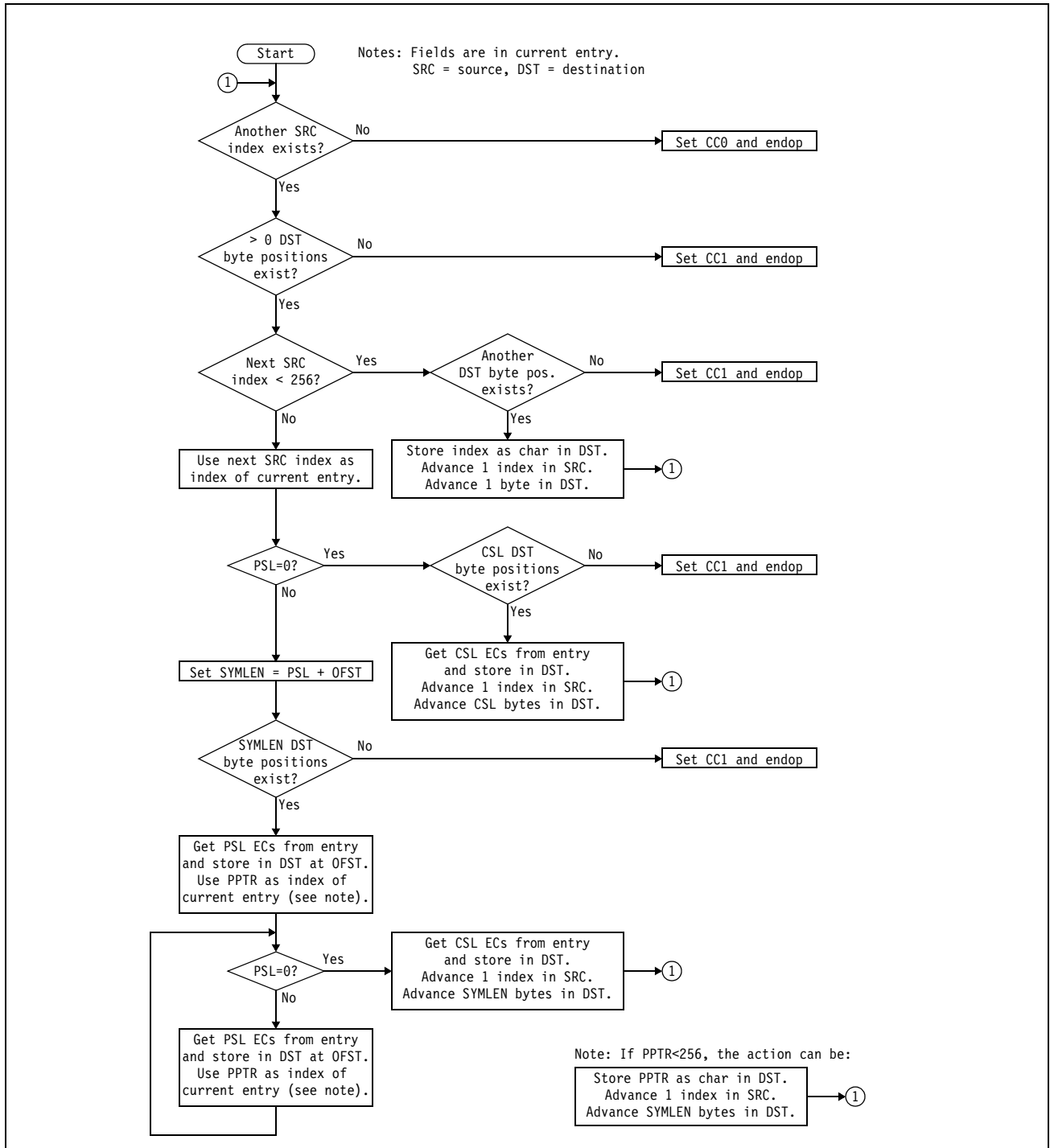
Figure 7-48. Expansion Process
