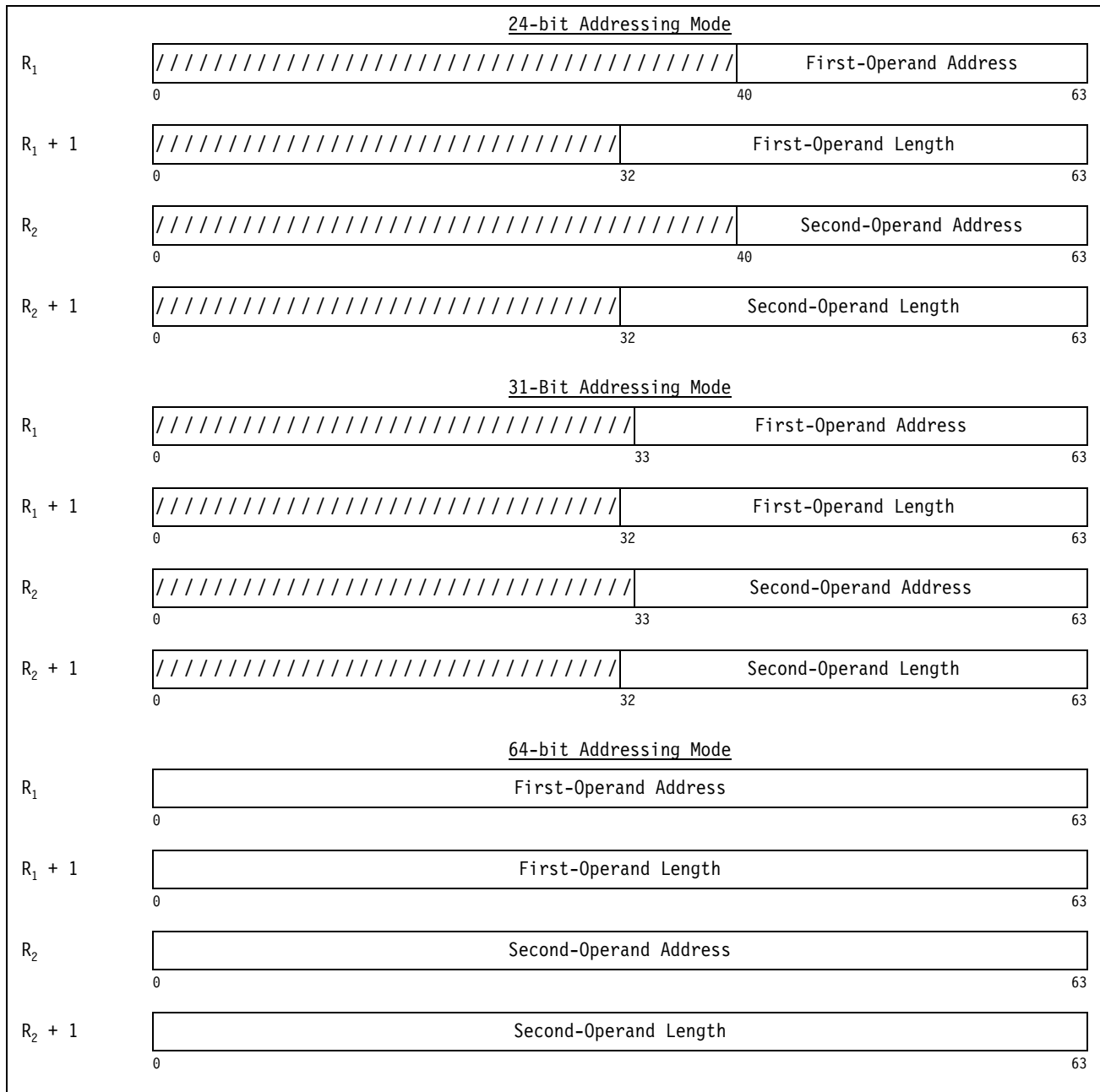
Figure 7-84. Register Contents for CONVERT UTF-16 TO UTF-8
