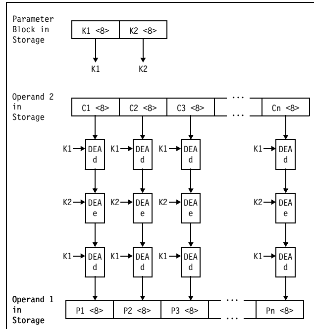
Figure 7-15. KM-TDEA-128 Decipher Operation
