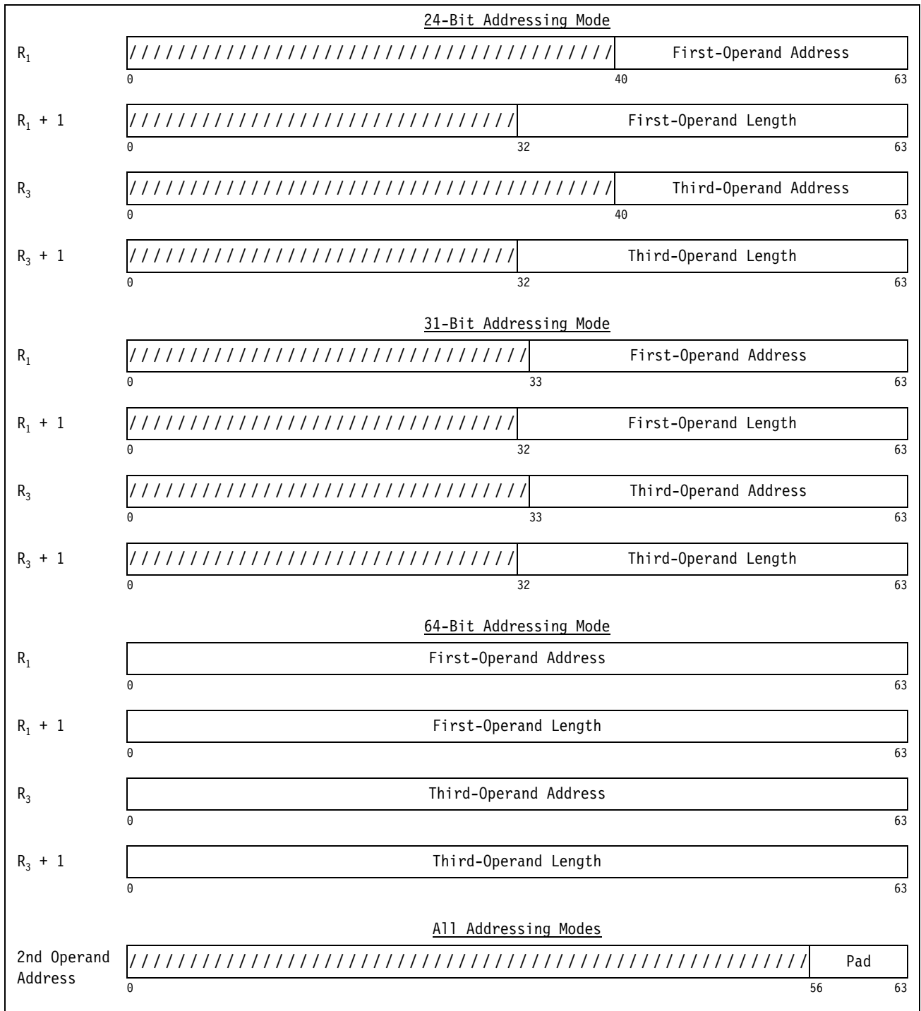
Figure 7-43. Register Contents and Second-Operand Address for COMPARE LOGICAL LONG EXTENDED
