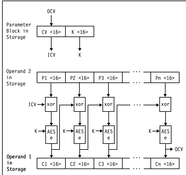
Figure 7-33. KMC-AES-128 Encipher Operation
