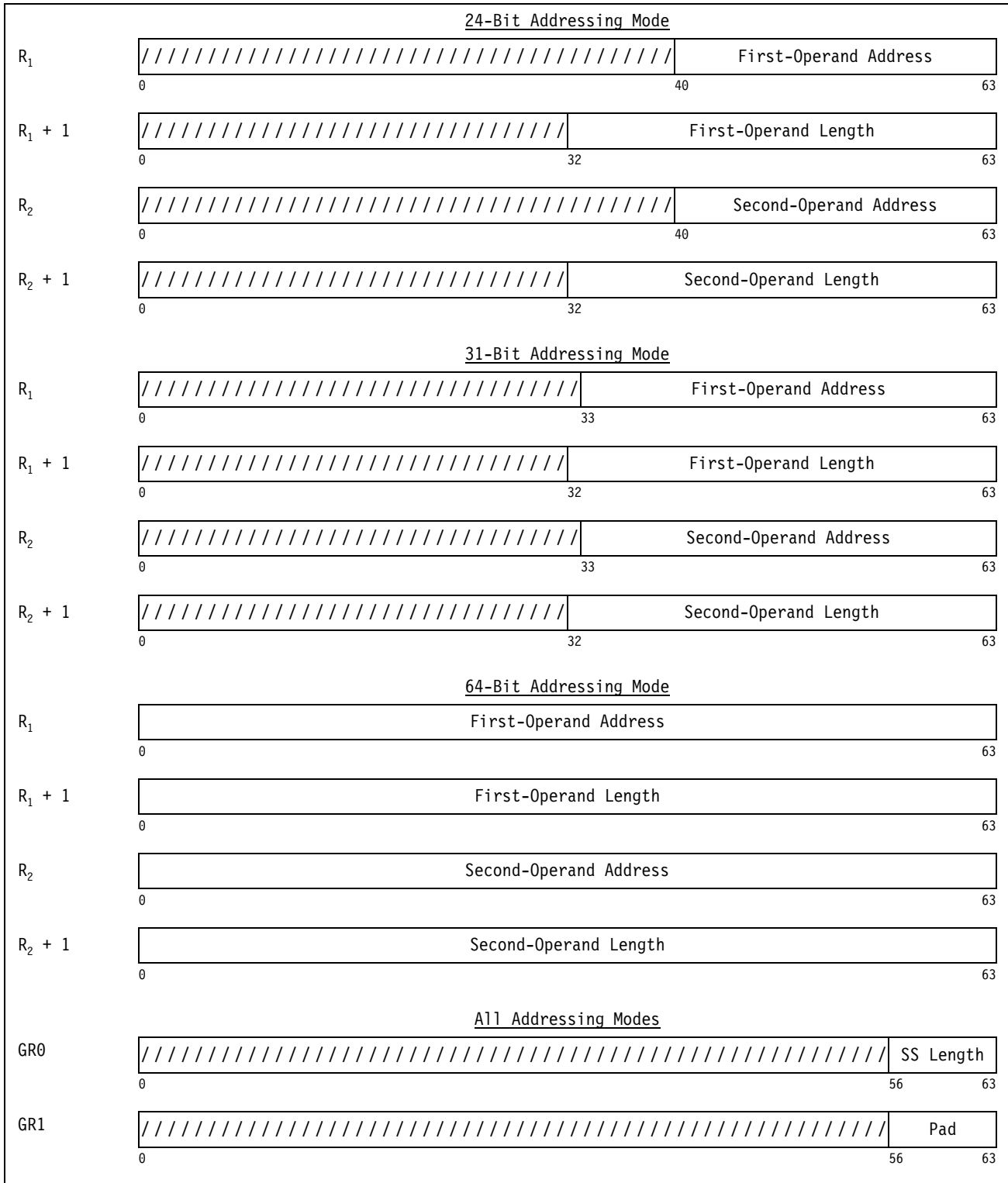
Figure 7-45. Register Contents for COMPARE UNTIL SUBSTRING EQUAL
