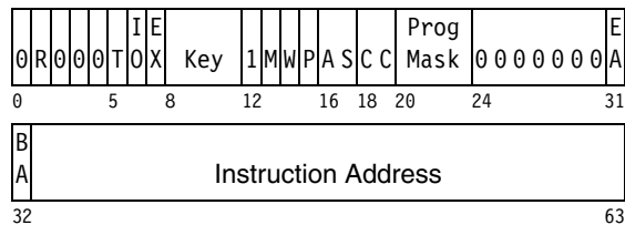
Figure 4-3. ESA/390 PSW Format, Except Bit 31 Shown as EA
