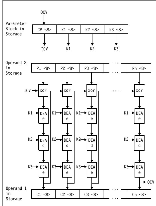
Figure 7-30. KMC-TDEA-192 Encipher Operation
