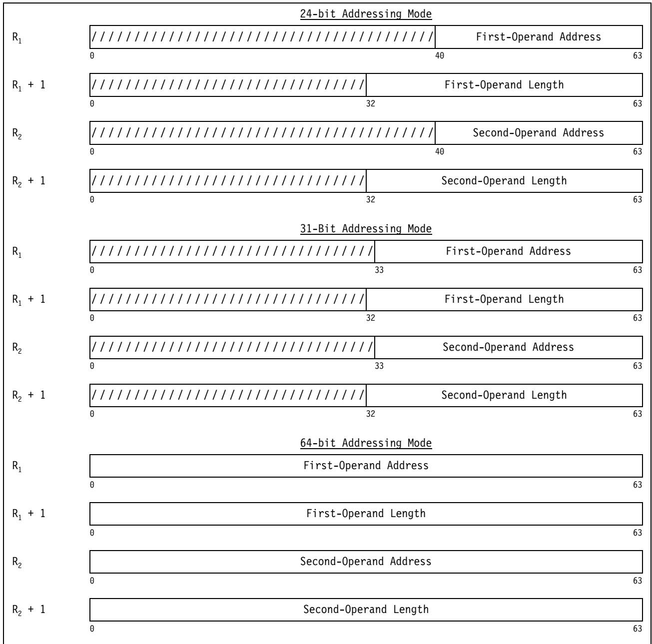
Figure 7-85. Register Contents for CONVERT UTF-32 TO UTF-16
