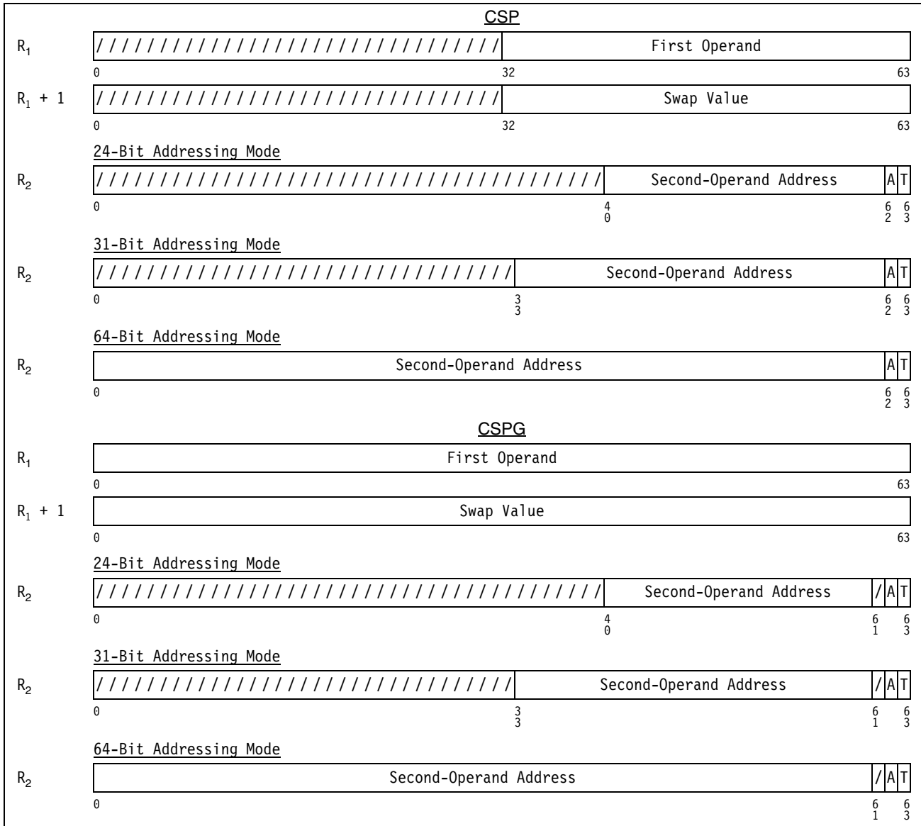
Figure 10-5. Register Contents for COMPARE AND SWAP AND PURGE
