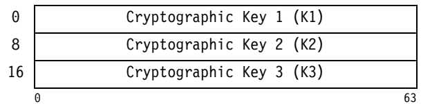
Figure 7-16. Parameter Block for KM-TDEA-192
