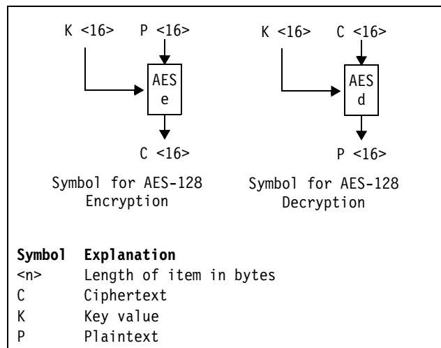
Figure 7-8. Symbols for AES-128 Encryption and Decryption
