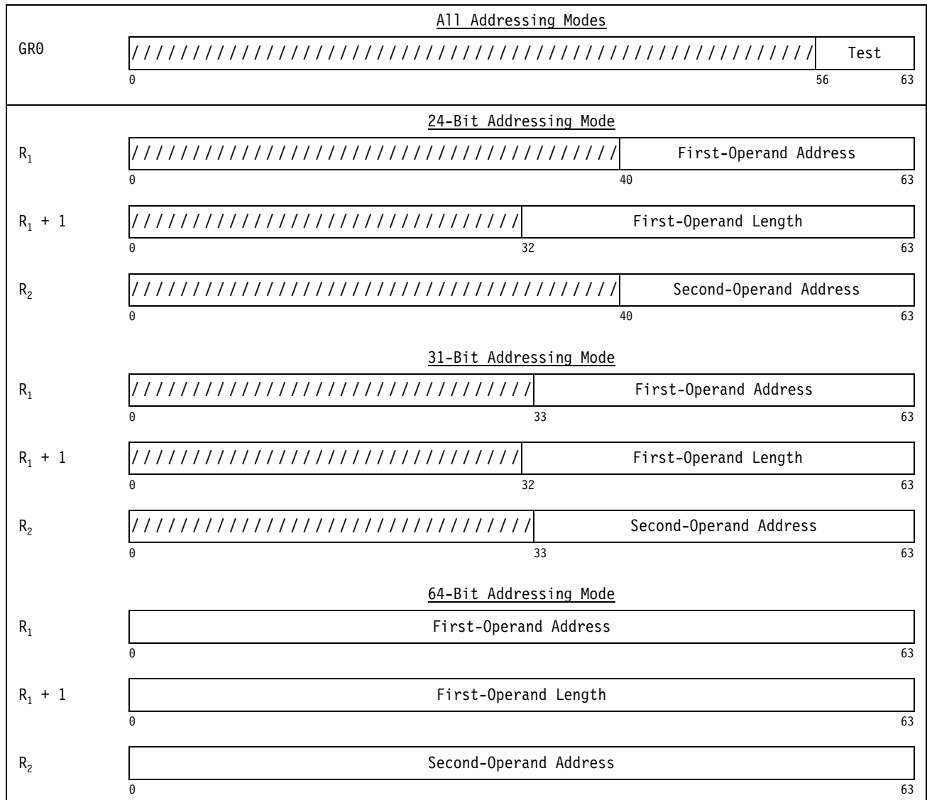
Figure 7-96. Register Contents for TRANSLATE EXTENDED
