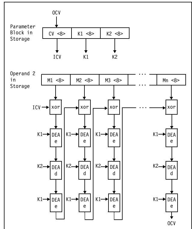
Figure 7-79. KMAC-TDEA-128
