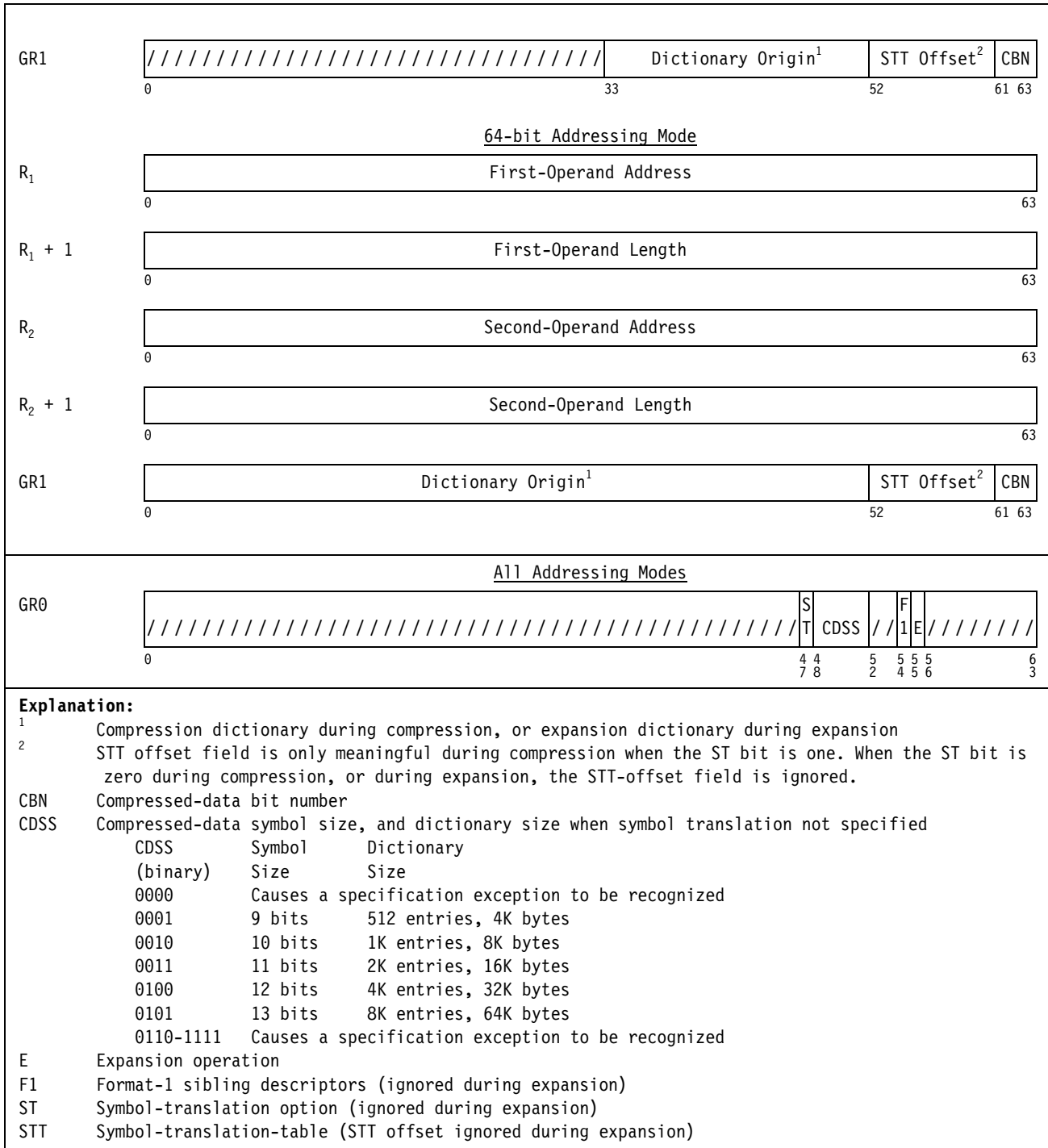
Figure 7-46. Register Contents for COMPRESSION CALL (Part 2 of 2)
