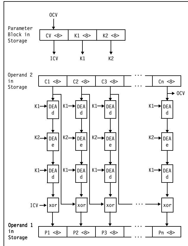
Figure 7-28. KMC-TDEA-128 Decipher Operation
