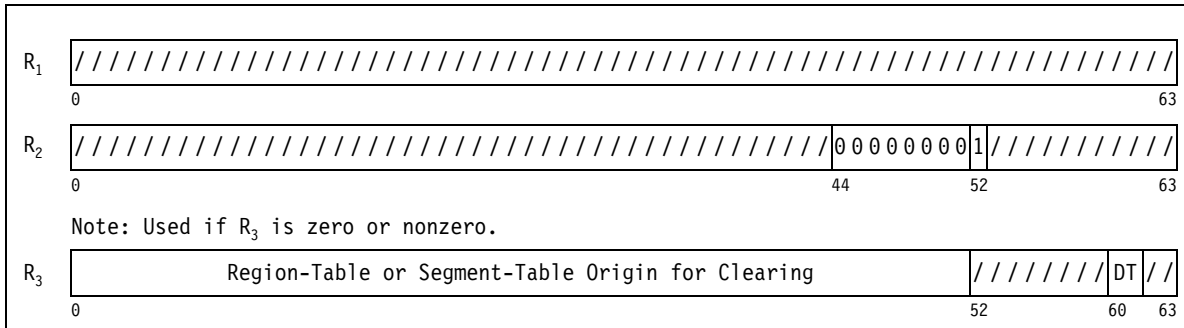
Figure 10-13. Register Contents for INVALIDATE DAT TABLE ENTRY Clearing-by-ASCE Operation (Bit 52 of GR R_2 Is One)
