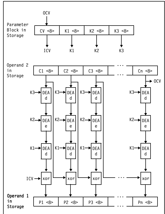
Figure 7-31. KMC-TDEA-192 Decipher Operation
