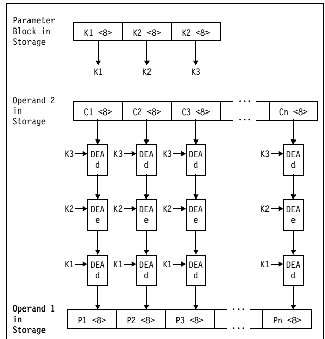
Figure 7-18. KM-TDEA-192 Decipher Operation
