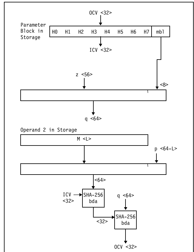
Figure 7-69. KLMD-SHA-256 Partial-Block Case 2 ( 56 \leq L \leq 63 )
