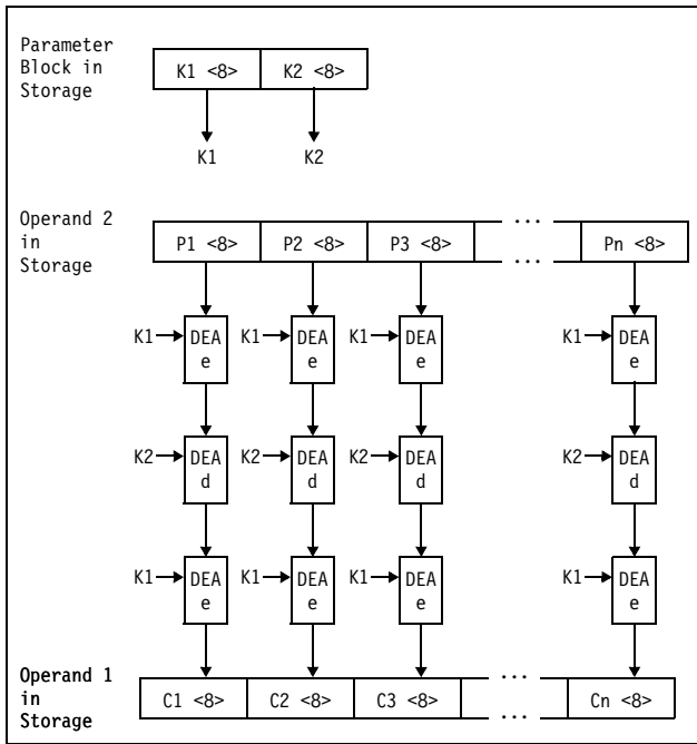
Figure 7-14. KM-TDEA-128 Encipher Operation
