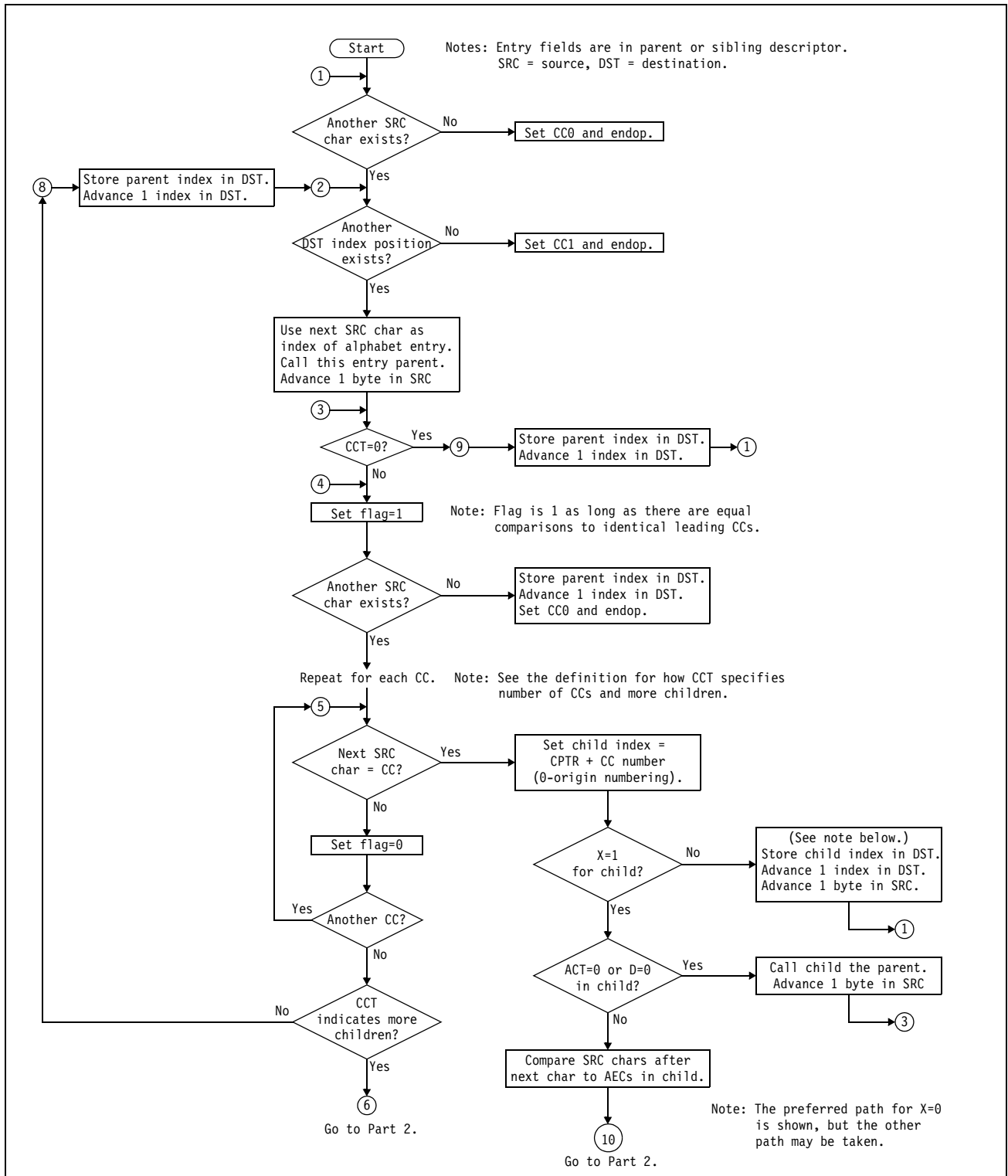
Figure 7-47. Compression Process (Part 1 of 2)
