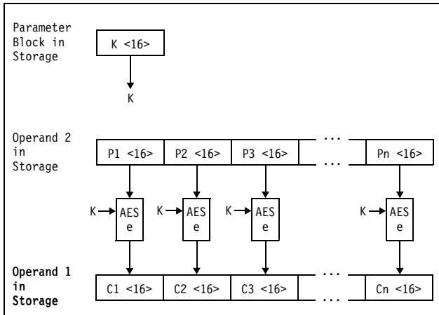
Figure 7-20. KM-AES-128 Encipher Operation
