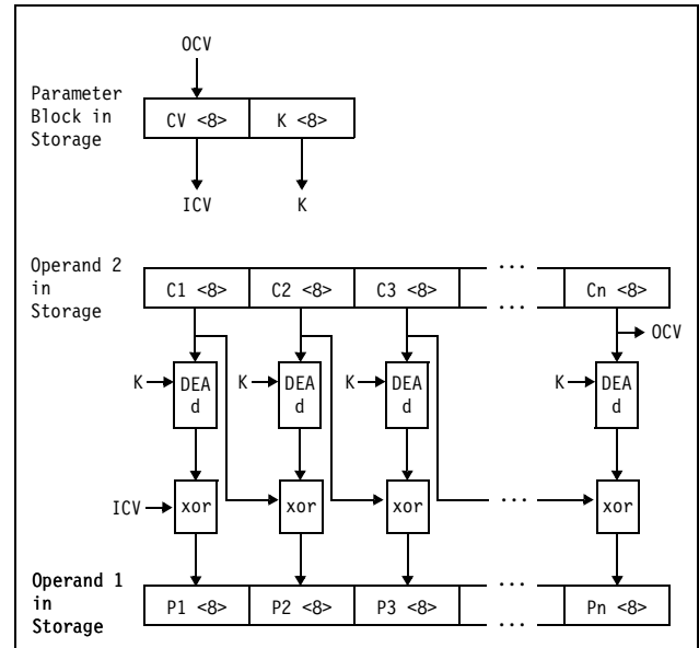
Figure 7-25. KMC-DEA Decipher Operation
