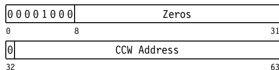
Format-1 TIC CCW
