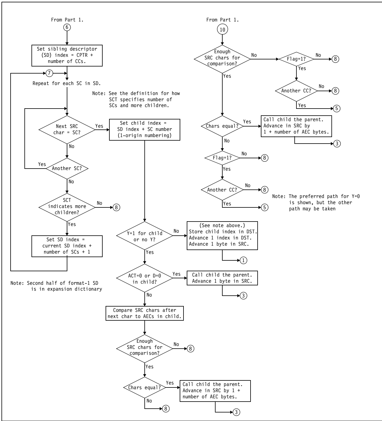
Figure 7-47. Compression Process (Part 2 of 2)
