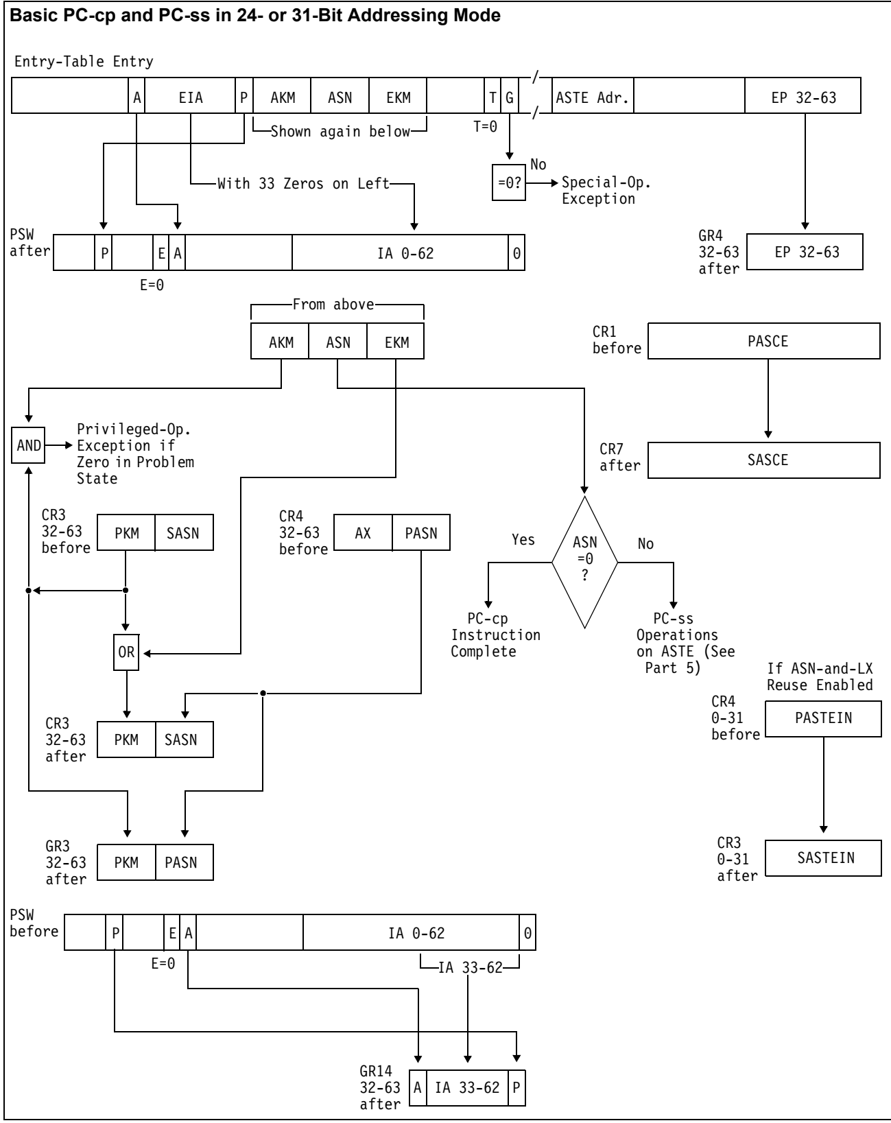
Figure 10-37. Execution of PROGRAM CALL (Part 1 of 5).
