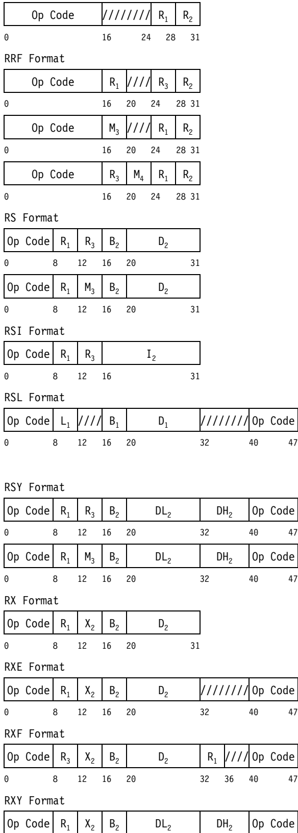
Figure 5-1. Basic Instruction Formats (Continued)
