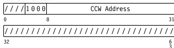
Format-0 TIC CCW
