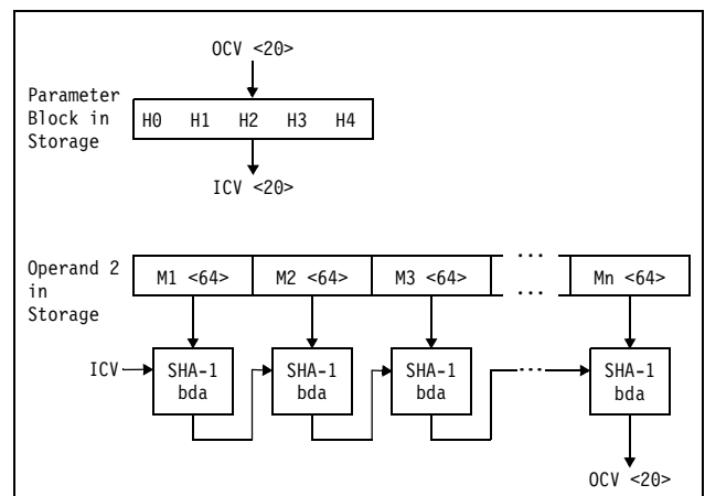
Figure 7-56. KIMD-SHA-1
