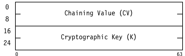
Figure 7-32. Parameter Block for KMC-AES-128
