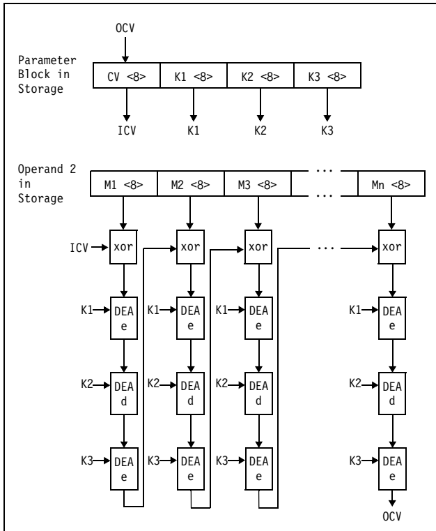
Figure 7-81. KMAC-TDEA-128
