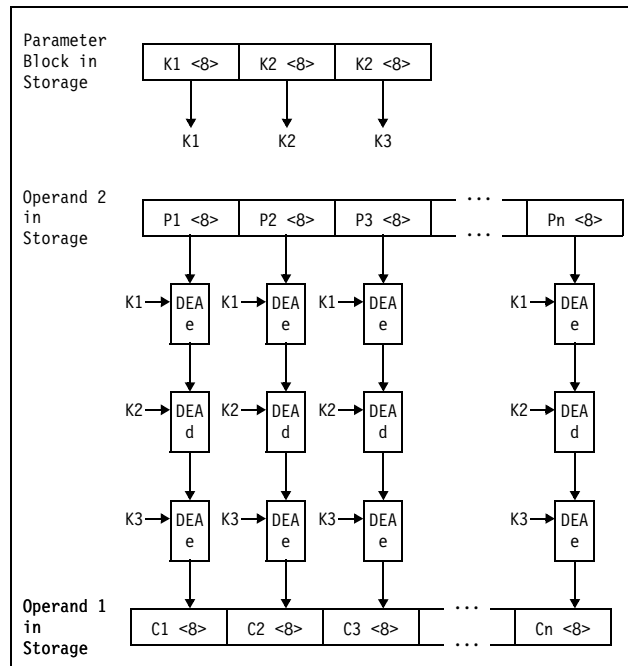
Figure 7-17. KM-TDEA-192 Encipher Operation
